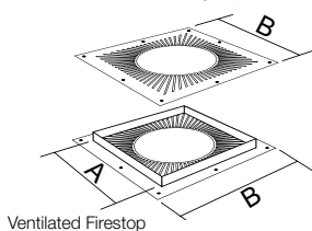
Ventilated Firestop
