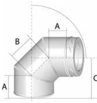
90° Elbow
