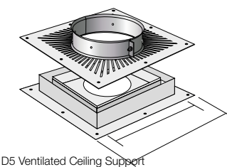
D5 Ventilated Ceiling Support
