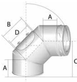
Inspection Elbow
