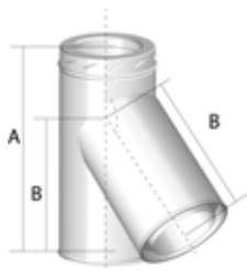
135° Tee & Elbow
