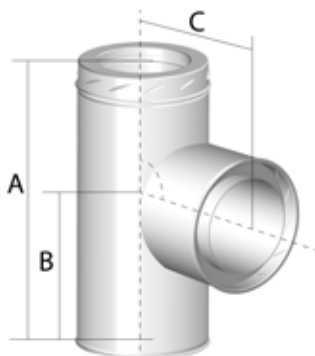
93° & 95° Equal Tee
