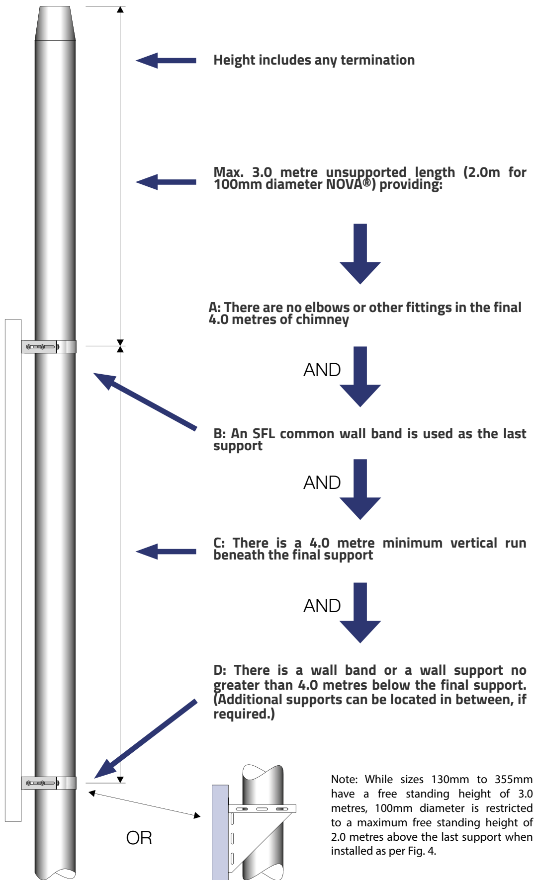
Fig. 4 Maximum unsupported termination detail
