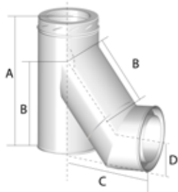
135° Tee & Elbow
